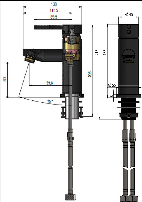
PINLESS HANDLE
